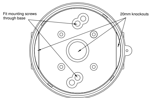
Fig 2 Mounting Beacon Base.
