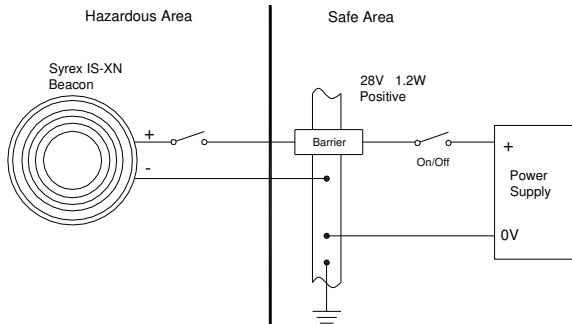
Fig 3 Using a single channel barrier.
